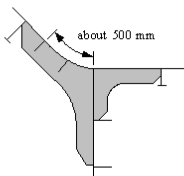
Figure 7: Example of insertion of horizontal gusset or longitudinal rib
