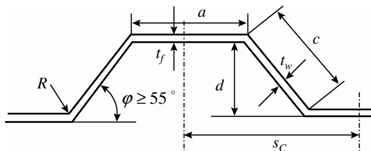
Figure 2: Corrugated bulkhead
