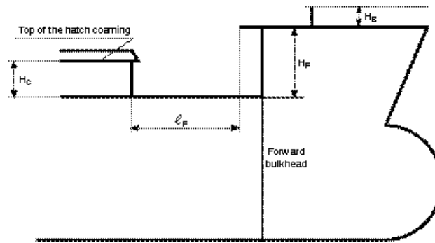
Figure 2: Forecastle
