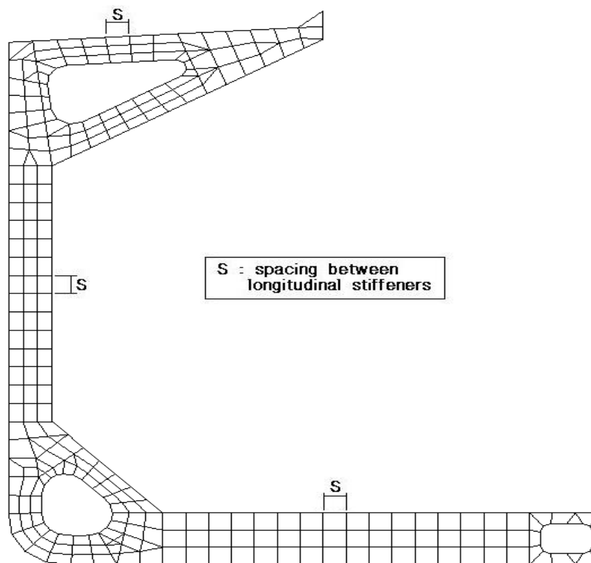
Figure 3: Typical mesh of a web frame
